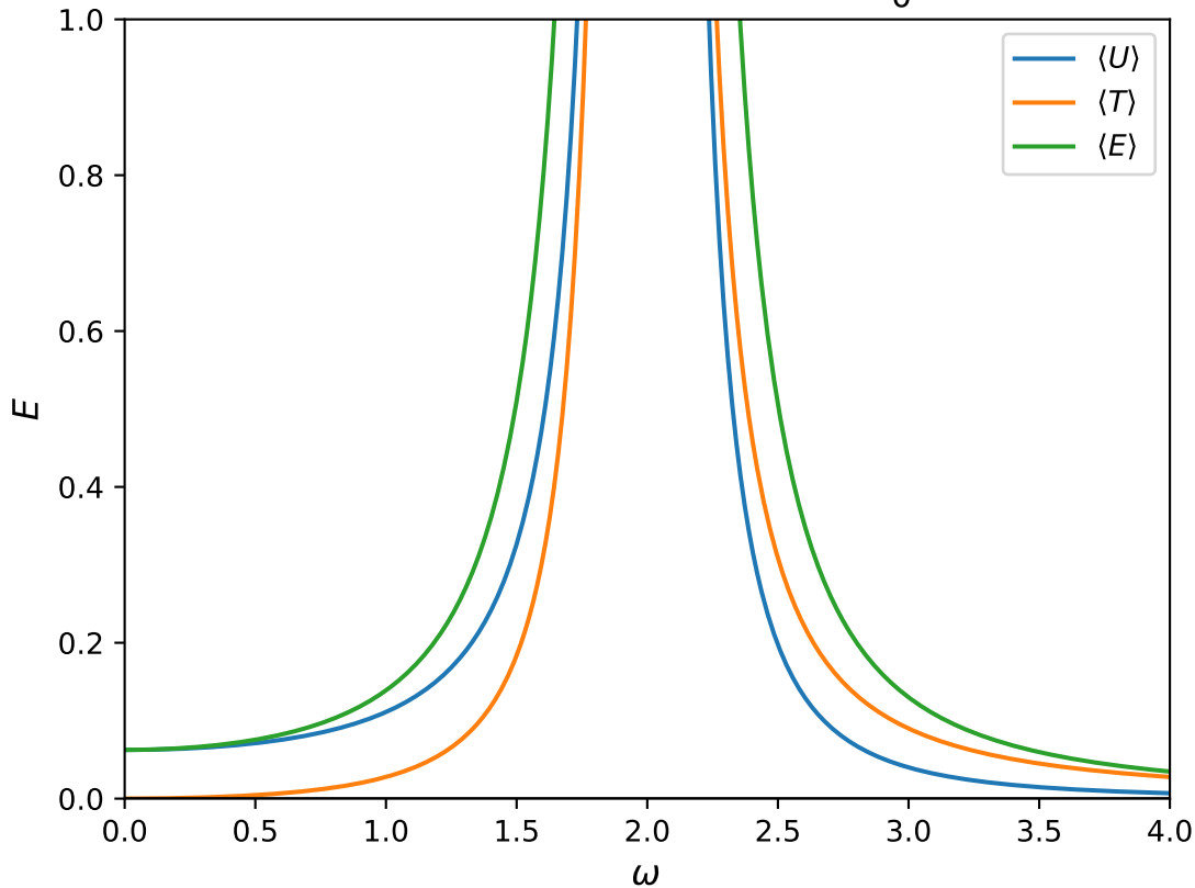
U and T versus \omega when \omega_0 = 2
